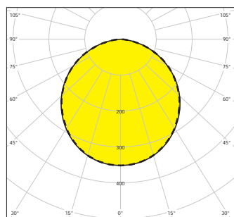
MAWERICK-LED-4K, IP20
