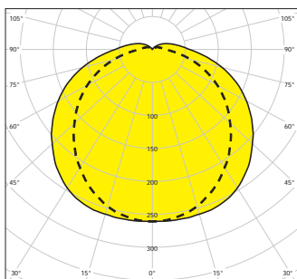
POINTER-LED-4K, IP66
